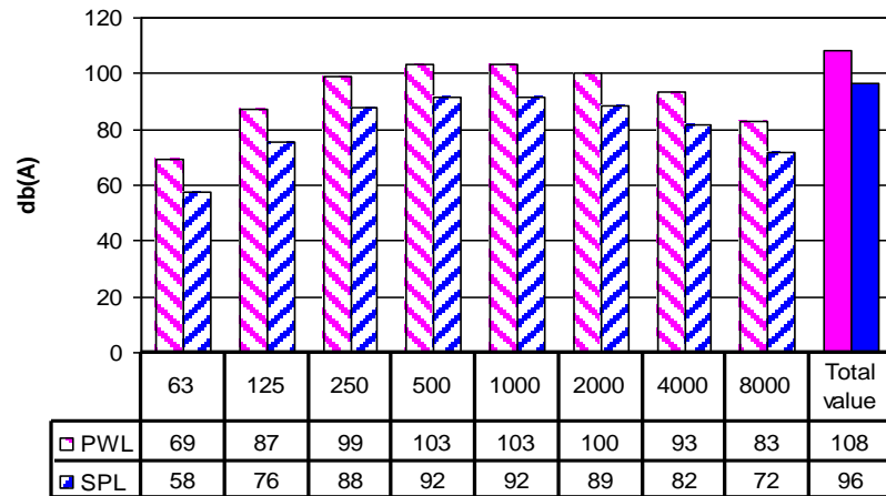
AF24-1600-8 RPM 960 20 °C
