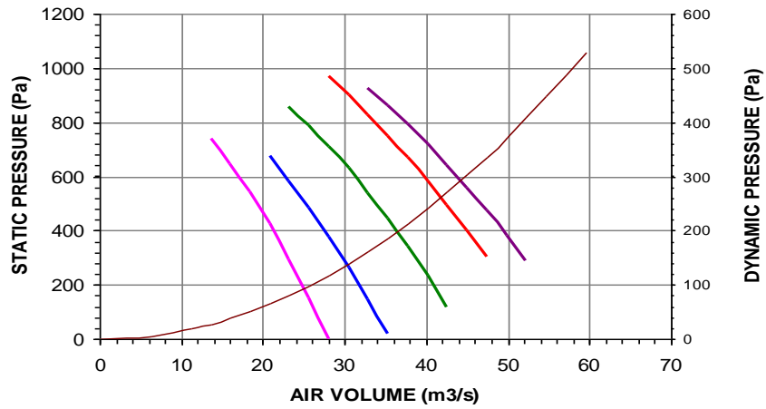
AF24-1600-8 RPM 960 20 °C
